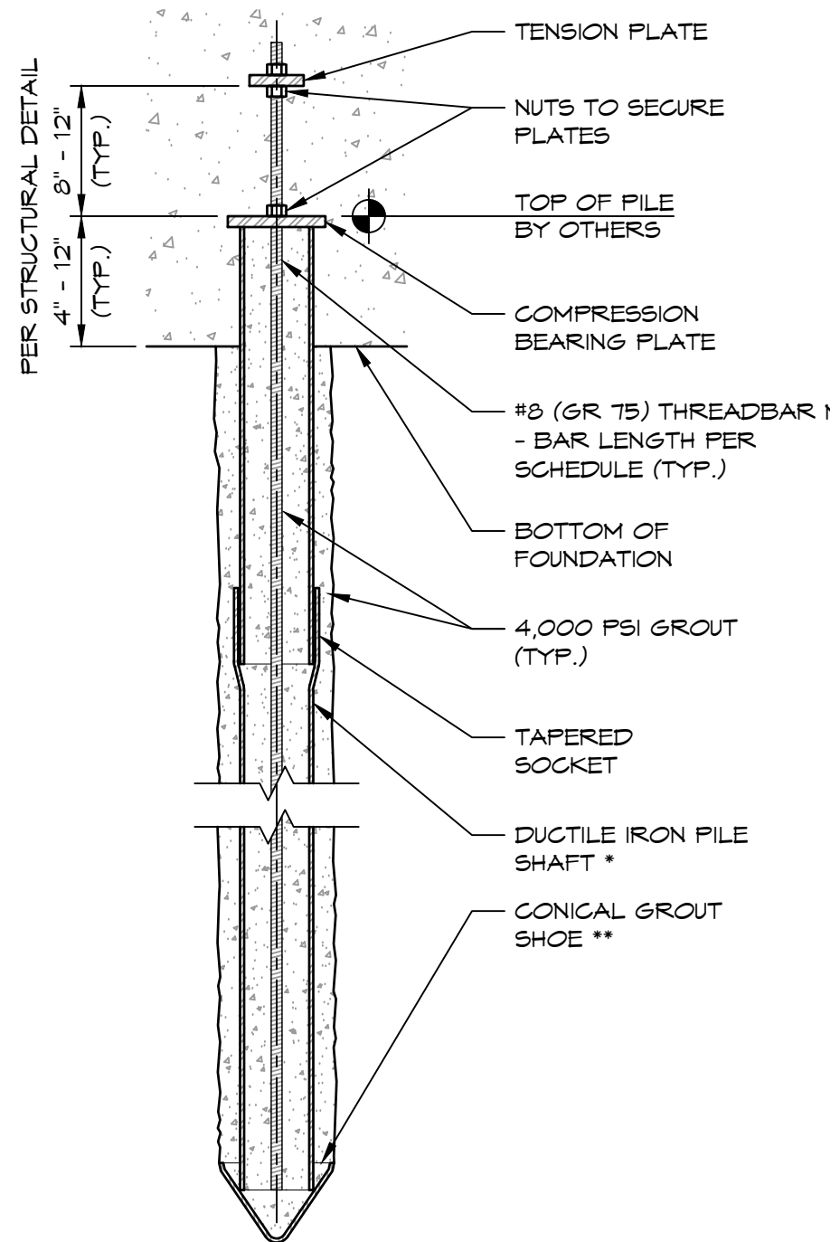
COMPRESSION / TENSION PILE
