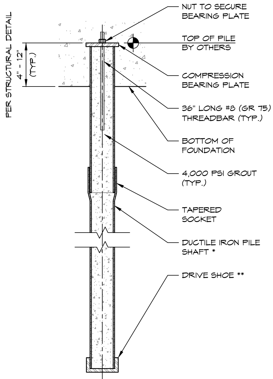
COMPRESSION PILE
