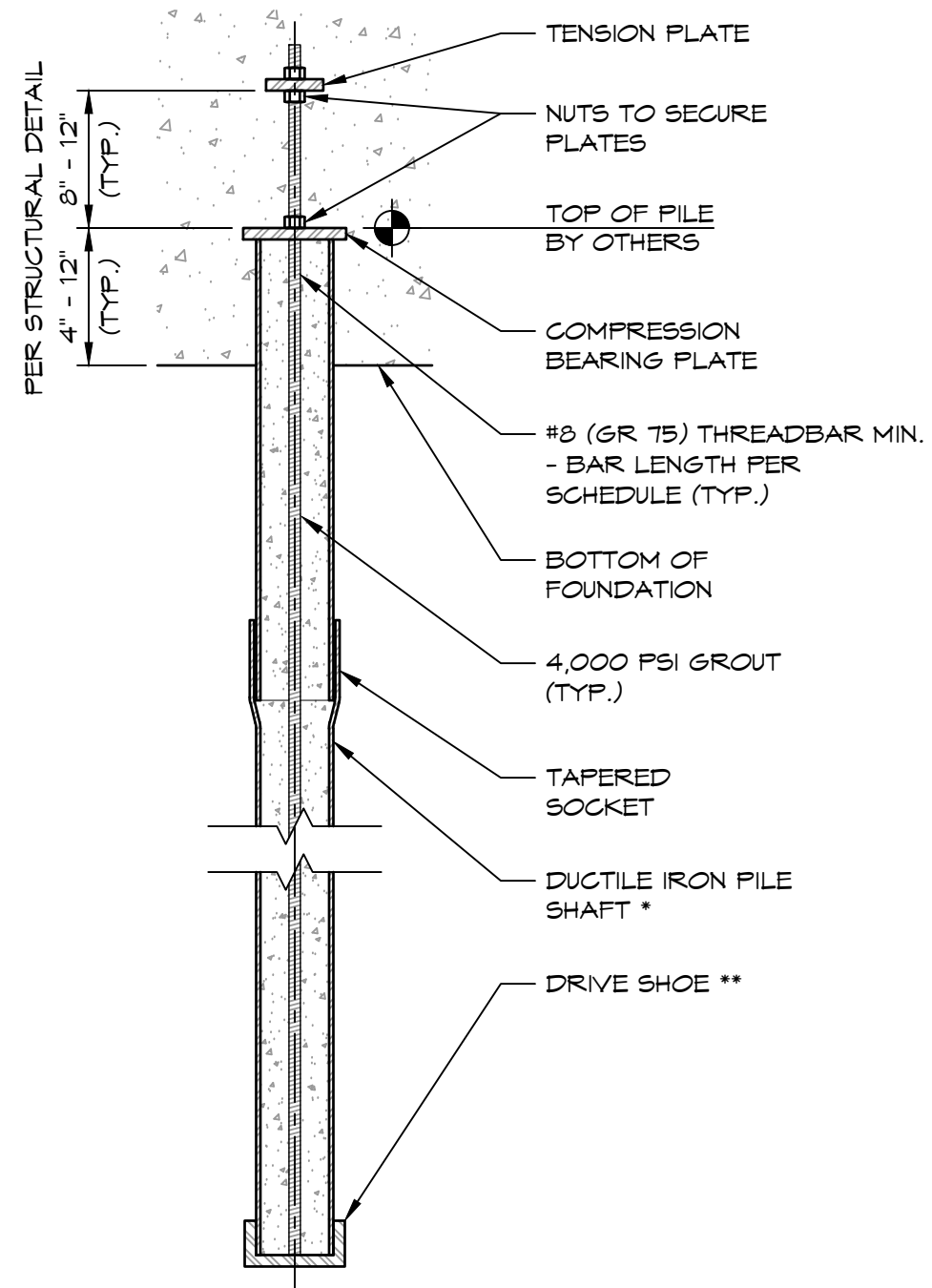
COMPRESSION / TENSION PILE
