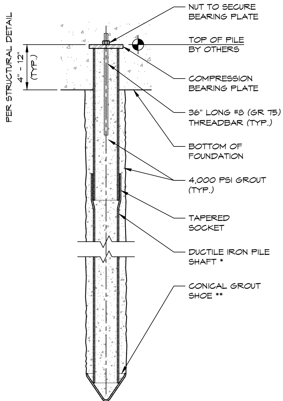
COMPRESSION PILE
