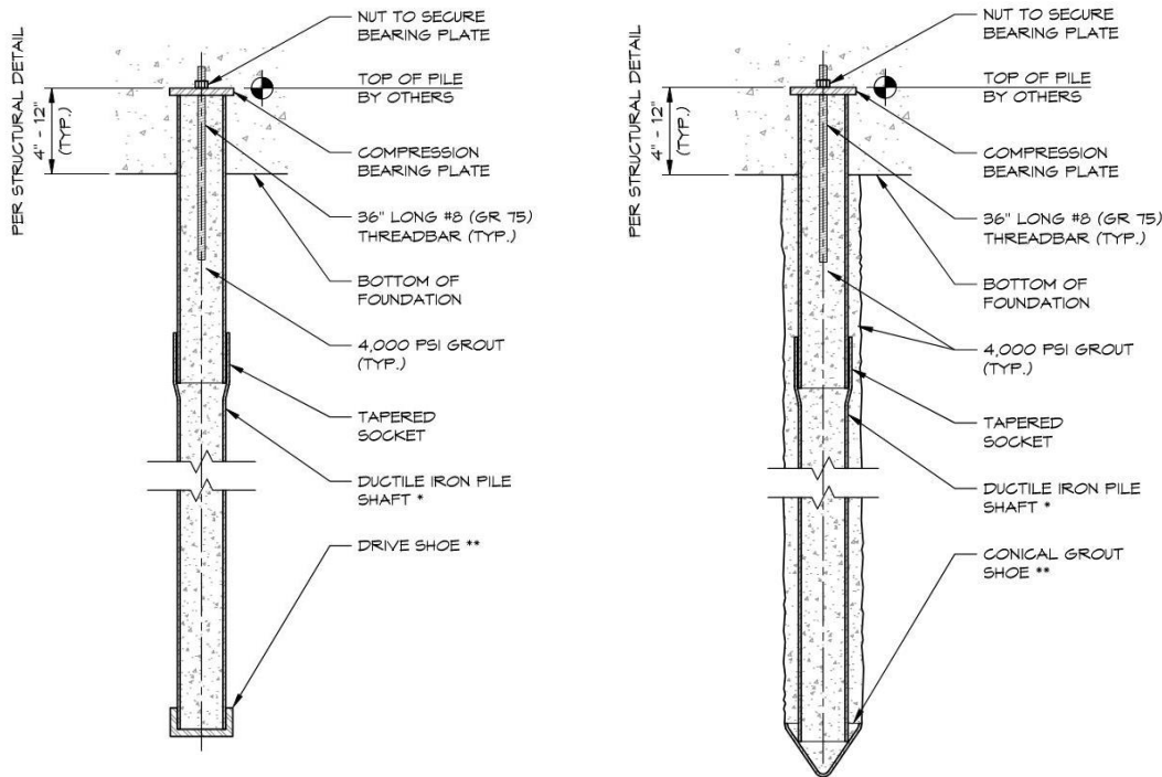
Figure 2: Examples of Ductile Iron Pile Details for Compression Loading
