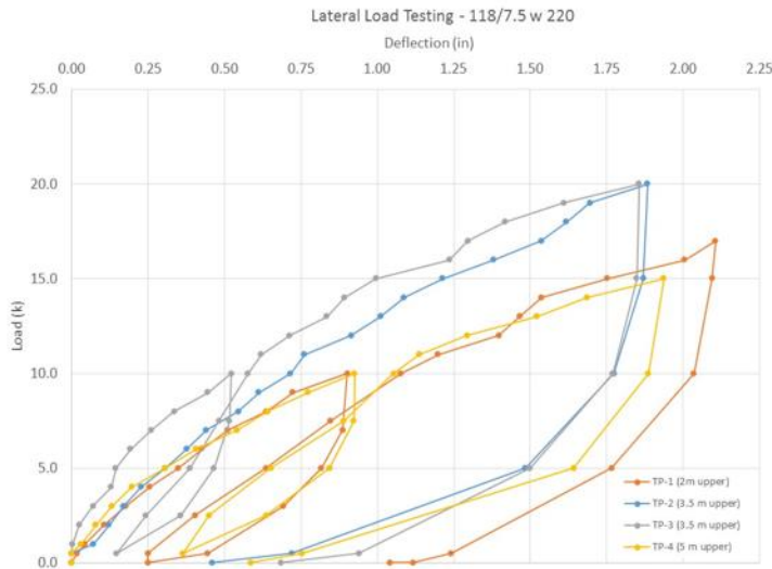
Figure 8: Full-scale Lateral Load Test Results on Series 118/7.5 with 220 mm Grout Shoe
