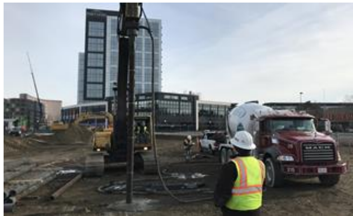
Figure 1: Ductile Iron Pile Installation
