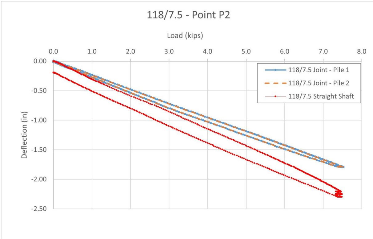
Figure 7: Ductile Iron Pile Bending Test Results
