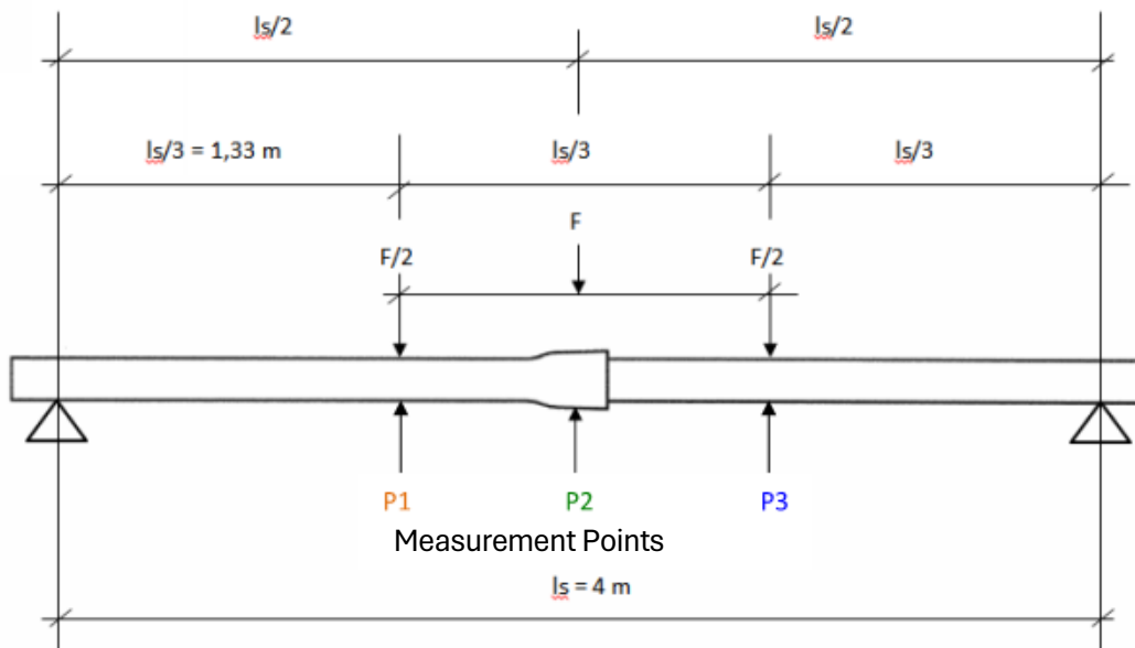
Figure 6: Schematic of Ductile Iron Pile Bending Test Setup (Austria)
