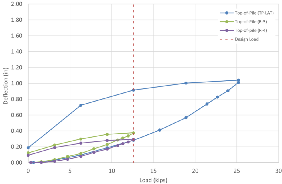
Figure 9: Full-scale Lateral Load Test Results including Reaction Piles on Series 170/9.0
