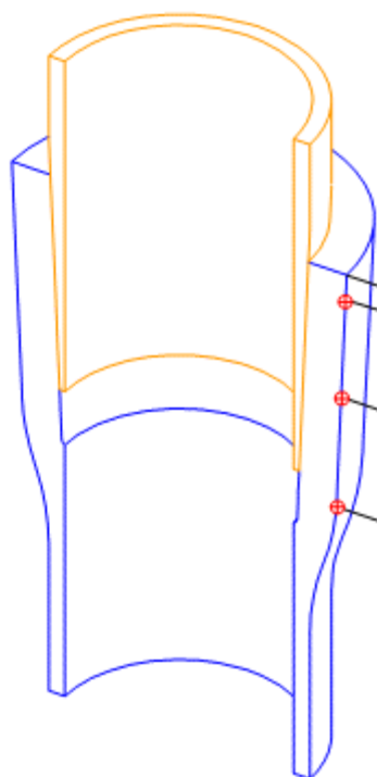
Figures 3a, b: Cross-section of Bell-Spigot Pile Socket and Laboratory Test Setup (Niederwanger and Lehar, 2001)
