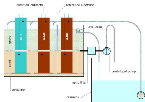
Figure 2: Schematic of Test Setup
