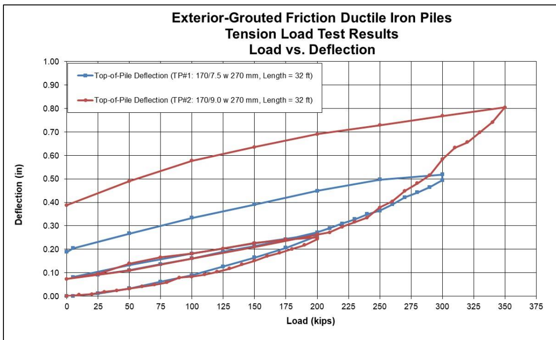
Figure 5: Tension Load Test Results for Exterior-Grouted Friction Ductile Iron Pile
