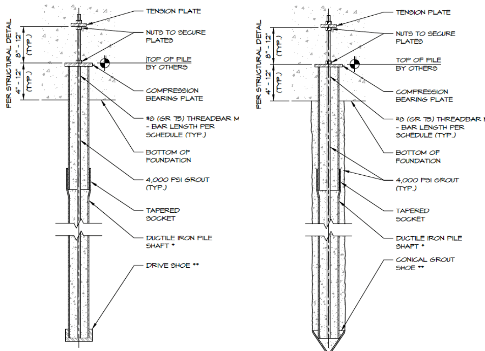
Figure 2: Examples of Ductile Iron Pile Tension Details – a) Non-grouted (Exterior) and b) Grouted (Exterior)
